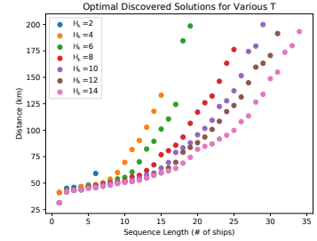
(c) Discovered Pareto-Optimal solutions for different time horizons T_F .
