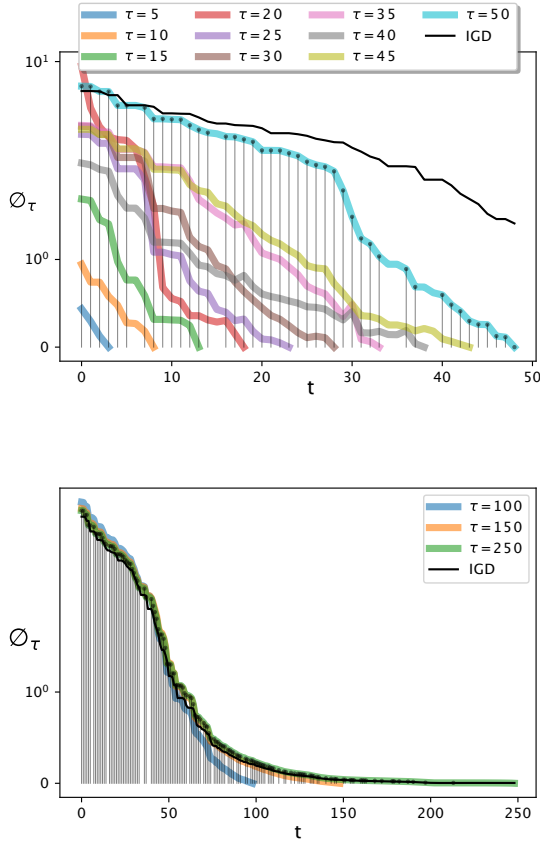
Fig. 7: Convergence of NSGA-II on ZDT6 during an early and a latter phase of the algorithm.
