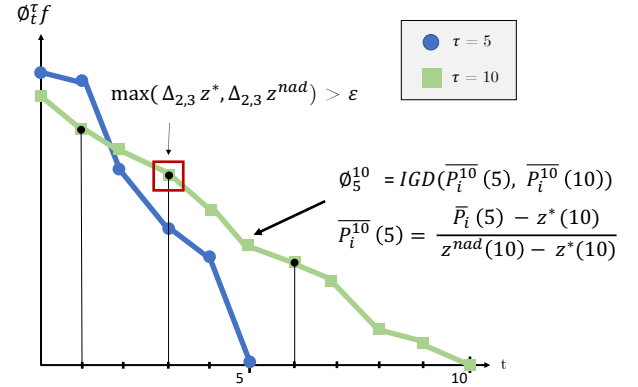
Fig. 4: Visualization of the running performance metric \emptyset_t^\tau at generations \tau = 5 and 10.
