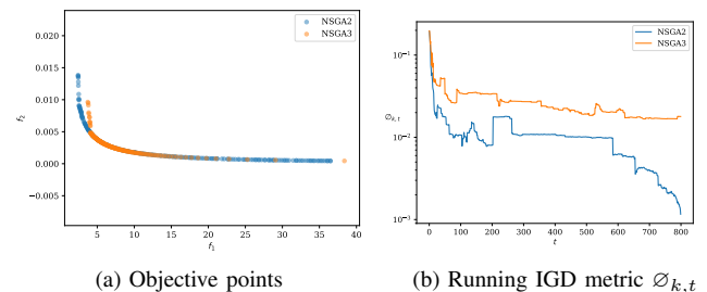
Fig. 8: Results on WELD problem (4 variables, 4 constraints, 2 objectives).
