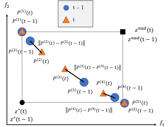
Fig. 2: A visualization of the average change in IGD values ( \varnothing_t ) from generation t-1 to t during the diversity phase \mathbb{C}^D .
